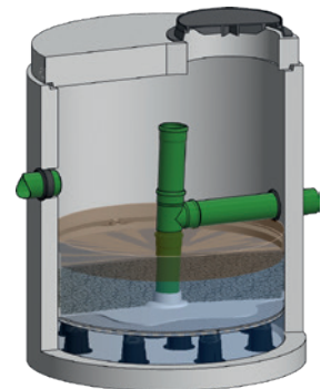
ViaGard F
