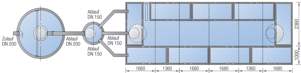
Sedimentationsanlage ViaSed
