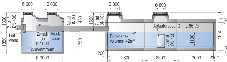
Sedimentationsanlage ViaSed
