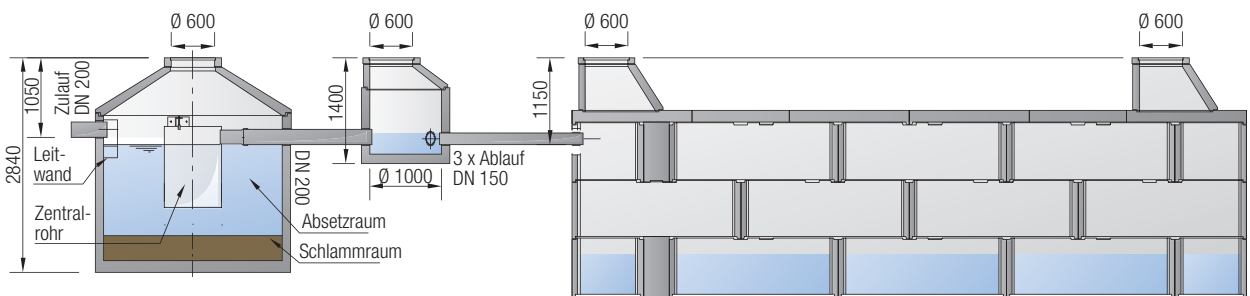
Sedimentationsanlage ViaSed
