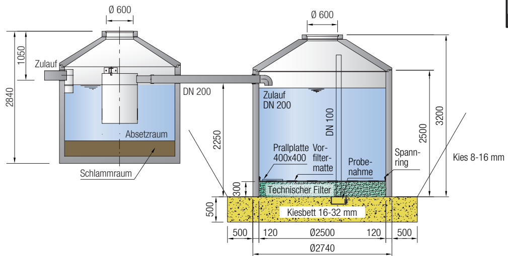
Sedimentationsanlage ViaSed
