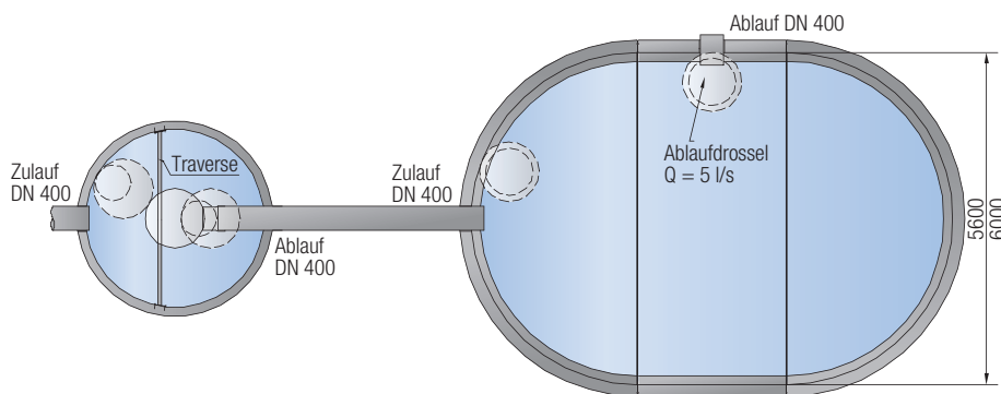
Sedimentationsanlage ViaSed
