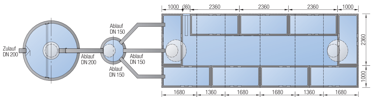
Sedimentationsanlage ViaSed
